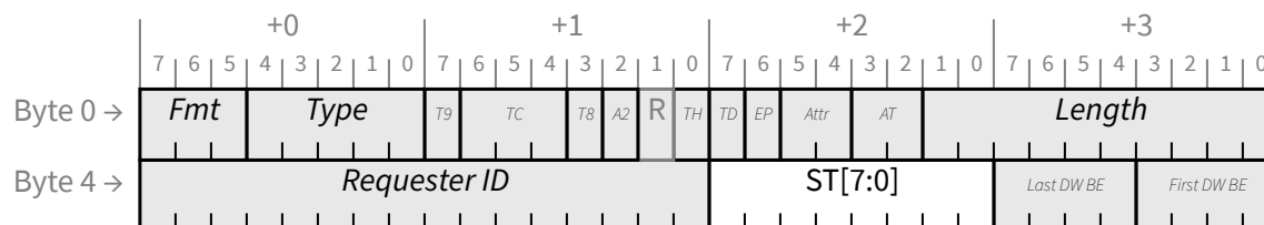
Figure 2-37 Location of ST[7:0] in the Memory Write Request Header - Non-Flit Mode
