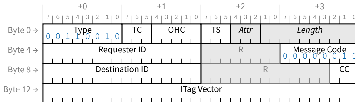
Figure 10-22 Invalidat Completion Message - Flit Mode
