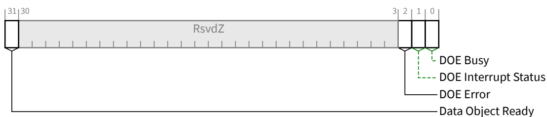
§ Figure 7-362 DOE Status Register
