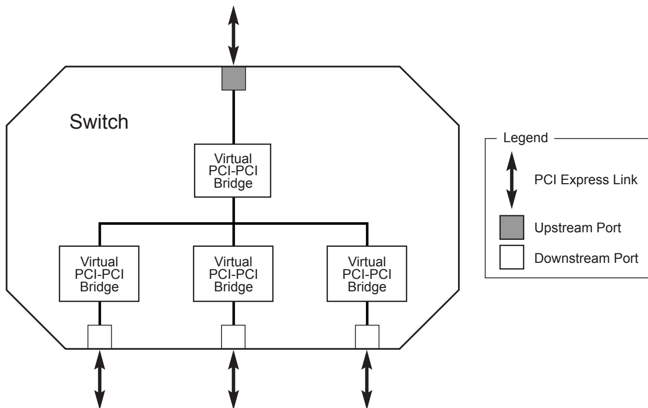
Figure 1-3 Logical Block Diagram of a Switch
